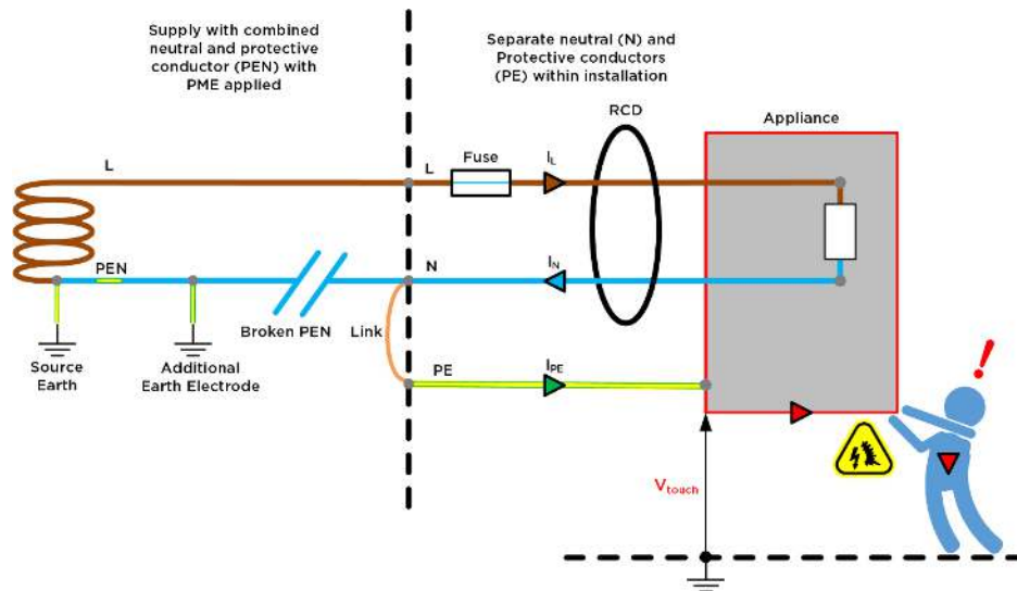
Figure 1: A break in the PEN conductor happens before the installation. No return path is available for the load current. V_{touch} > 0\text{ V} and can be dangerous. If a user connects PE and true earth by touching the metalwork, the load current will flow through the user: I_L = I_N = I_{PE} . The RCD does not trip and the user is in danger.
