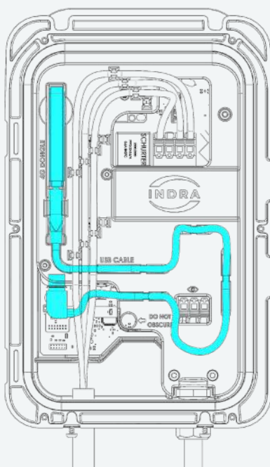
Figure 9: Smart LUX™ Dongle Routing
