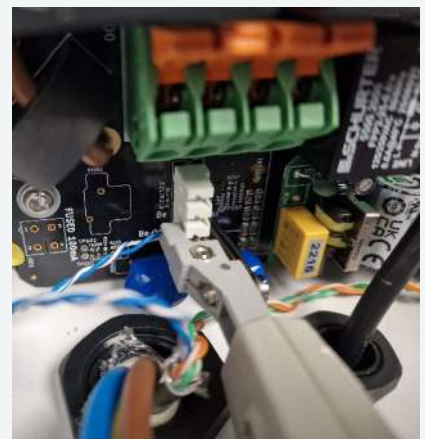
Figure 19: Charger CT Termination
