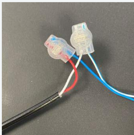
Figure 18: Data Cable Jelly Crimps
