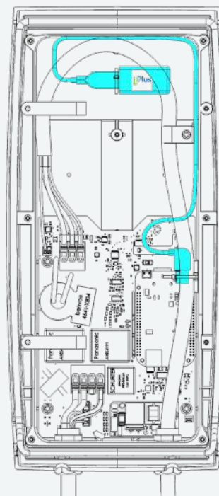
Figure 10: Smart PRO Dongle Routing
