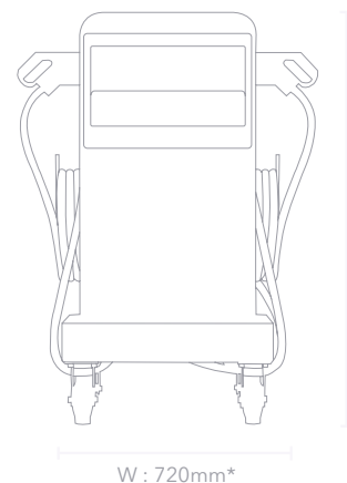
MAXICHARGER DC COMPACT PEDESTAL FRONT VIEW
