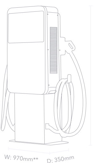
MAXICHARGER DC COMPACT PEDESTAL SIDE VIEW
